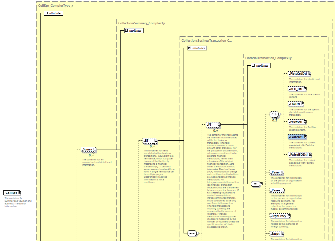
Figure 6: EDA Schema v5.0.3 - Picture for Detail Only
