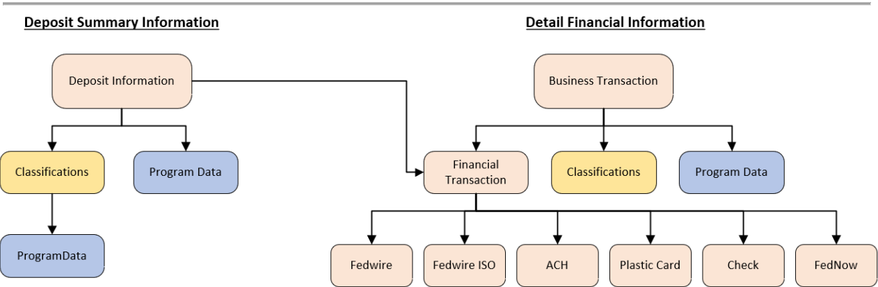
Figure 1: CIR Data Model
