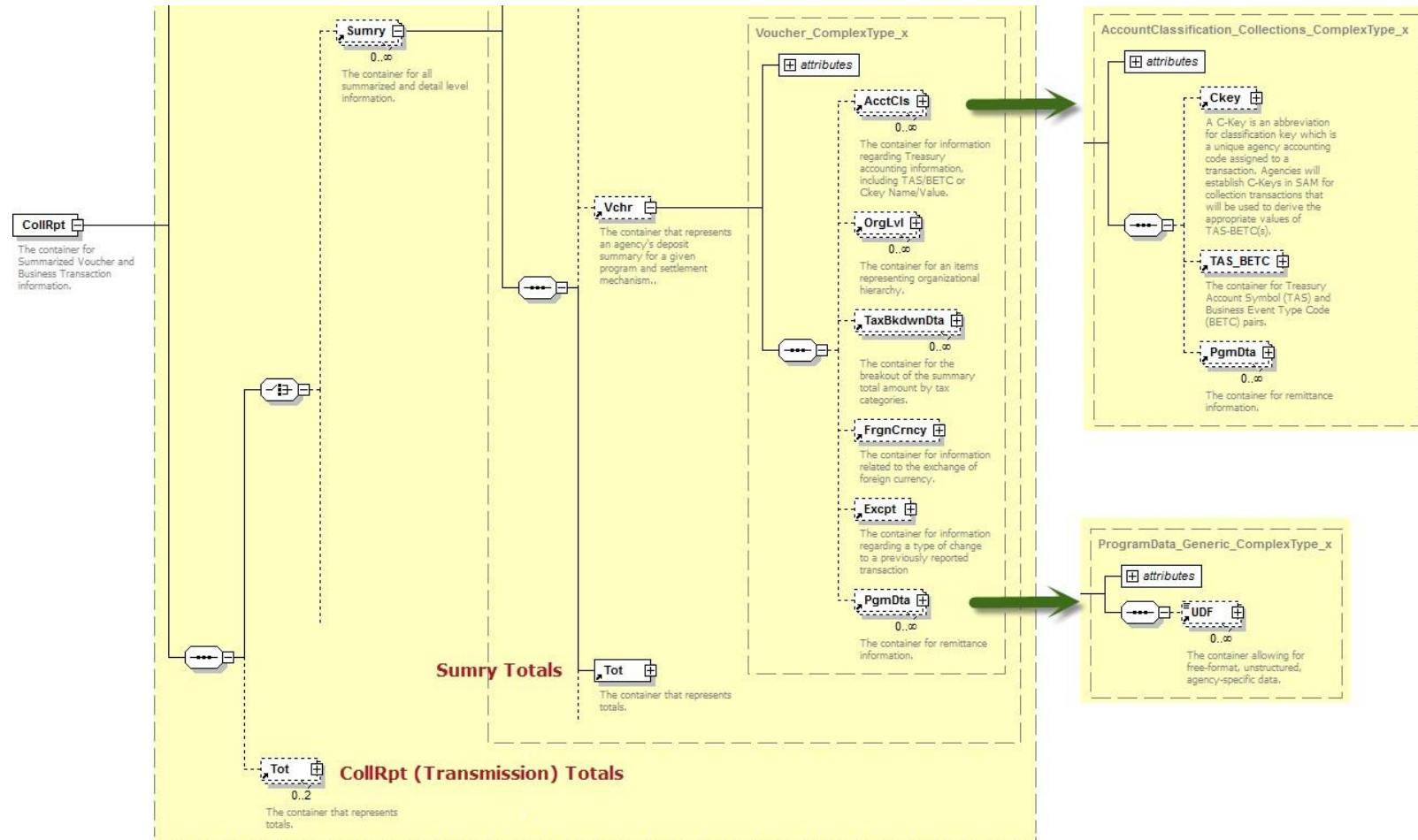
Figure 5: EDA Schema v5.0.3 - Picture for Summary Only Extract
