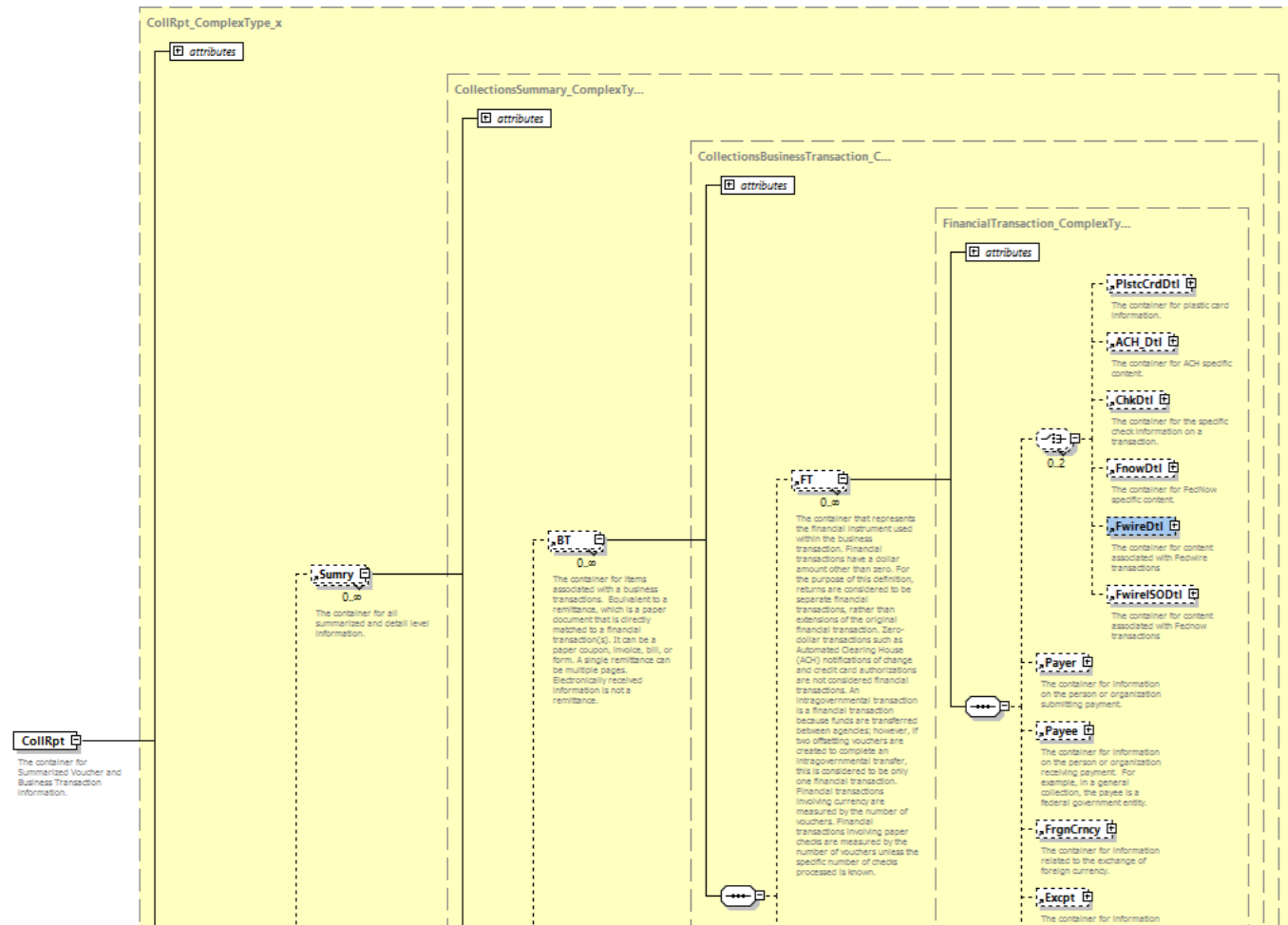
Figure 7: EDA Schema v5.0.3 - Picture for Summary and Detail
